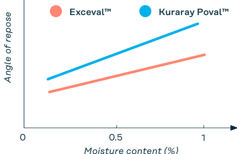
Fig.2 Angle of repose of spray dried ferrite particles
